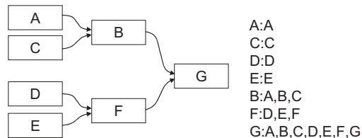
Figure 2: Justification and label structure resulting from (gen1M \text{ } B \text{ } A) (gen1MT \text{ } B \text{ } C) (gen1MT \text{ } F \text{ } D) (gen1MT \text{ } F \text{ } E) (gen1MT \text{ } G \text{ } B) (gen1MT \text{ } G \text{ } F) .
